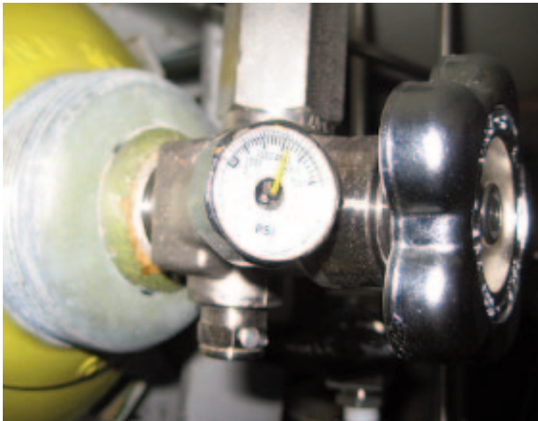
0-7,000 PSI GAUGE INSTALLED IN A MONEL VALVE
